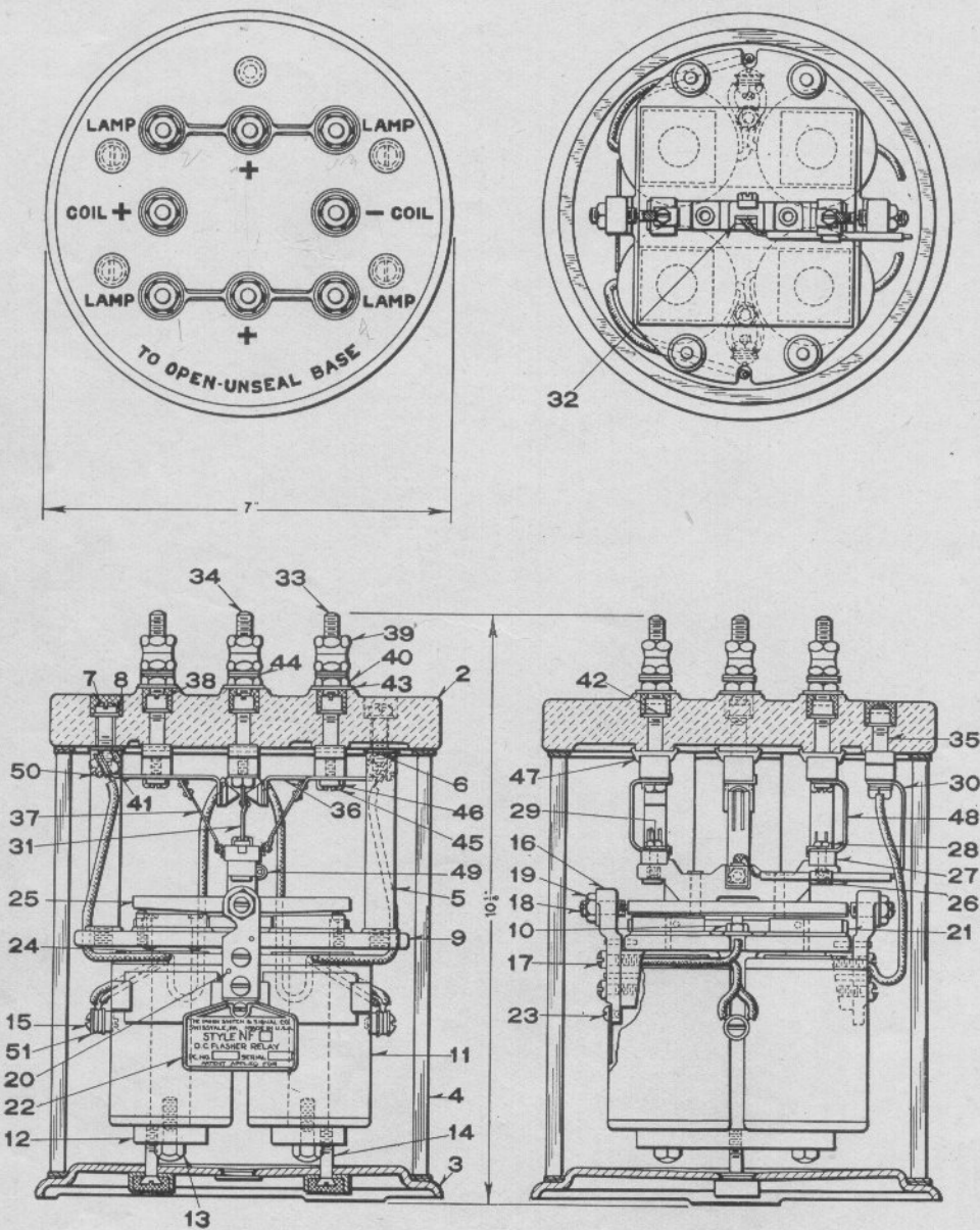
DETAILS OF THE STYLE "NF" D. C. FLASHER RELAY
