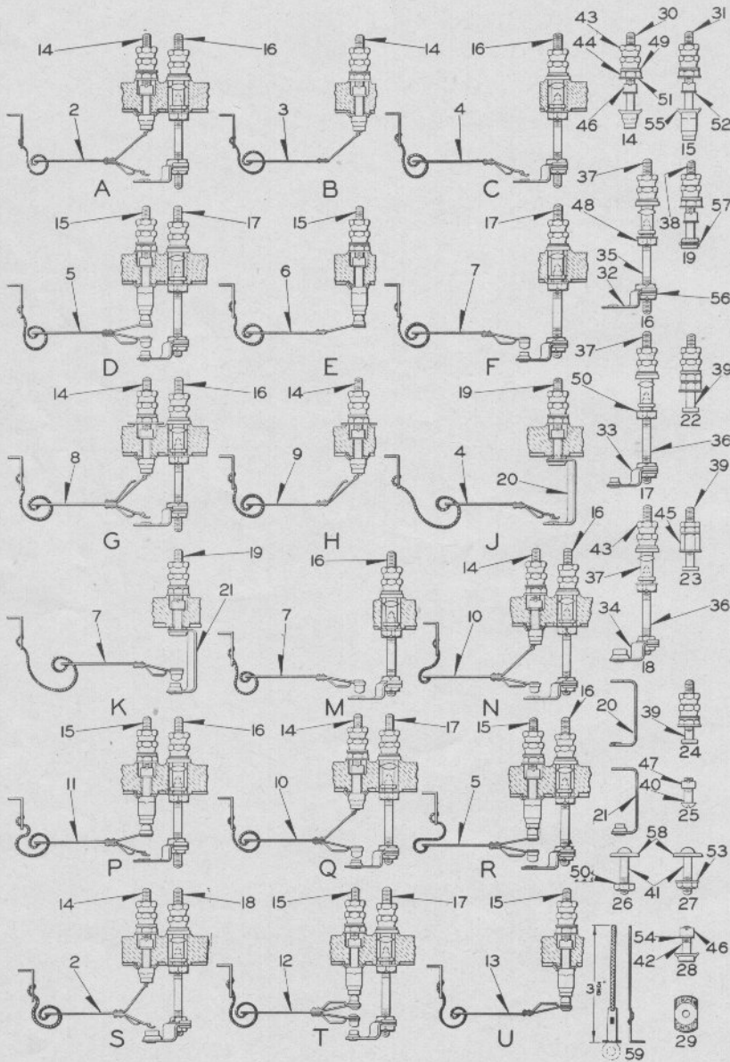
MODEL 12 DIRECT CURRENT ENCLOSED INTERLOCKING RELAY DETAIL PARTS
