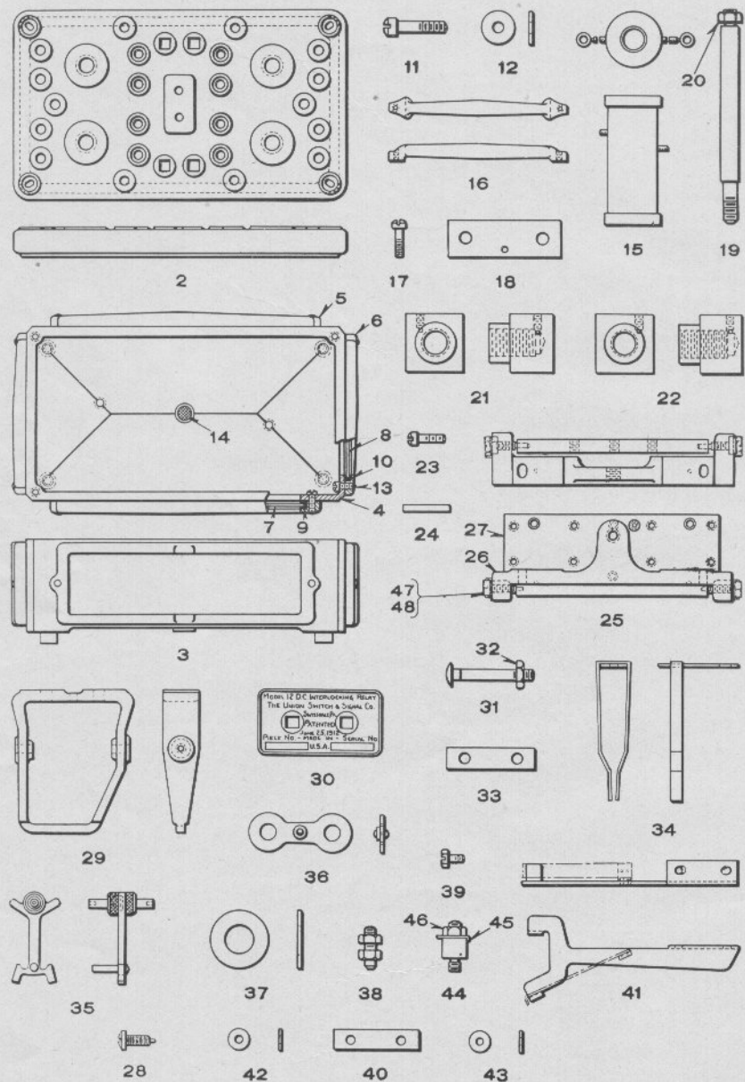
MODEL 12 DIRECT CURRENT ENCLOSED INTERLOCKING RELAY DETAIL PARTS
