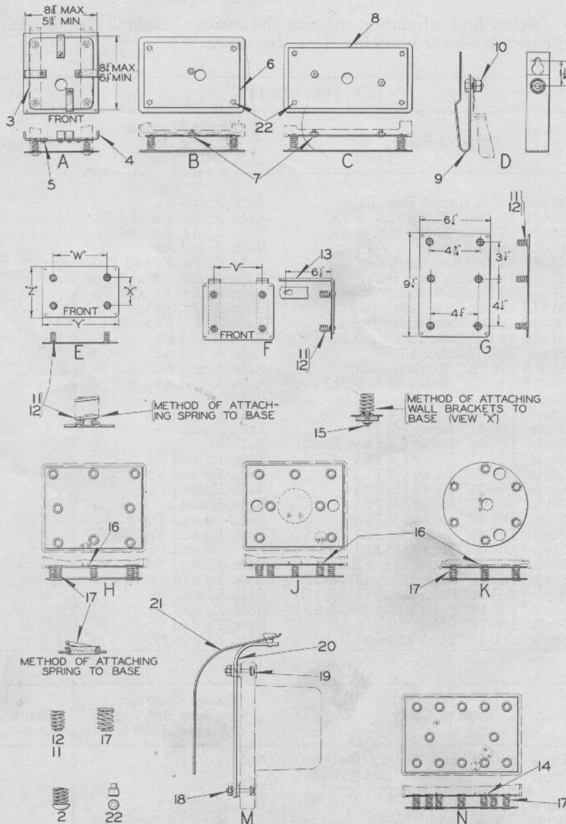
SHOCK ABSORBER SPRING BASES FOR D. C. AND A. C. RELAYS
