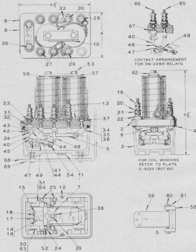
Styles "DN-22B" D. C. Biased Neutral Relay And "DN-22BH" D. C. Biased Neutral High Release Relay
