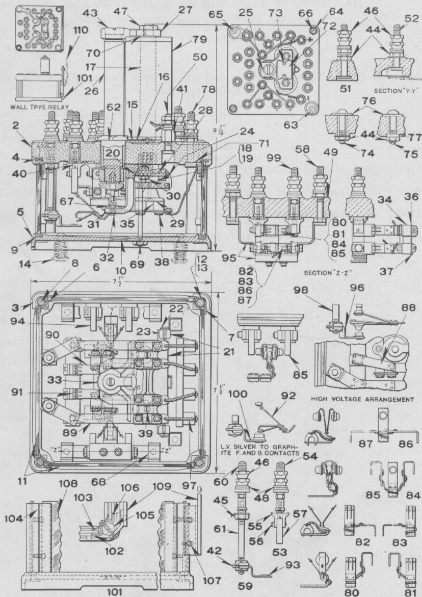
DETAILS OF MODEL 12 POLARIZED RELAY (FOUR NORMAL AND FOUR REVERSE POLAR CONTACTS)
