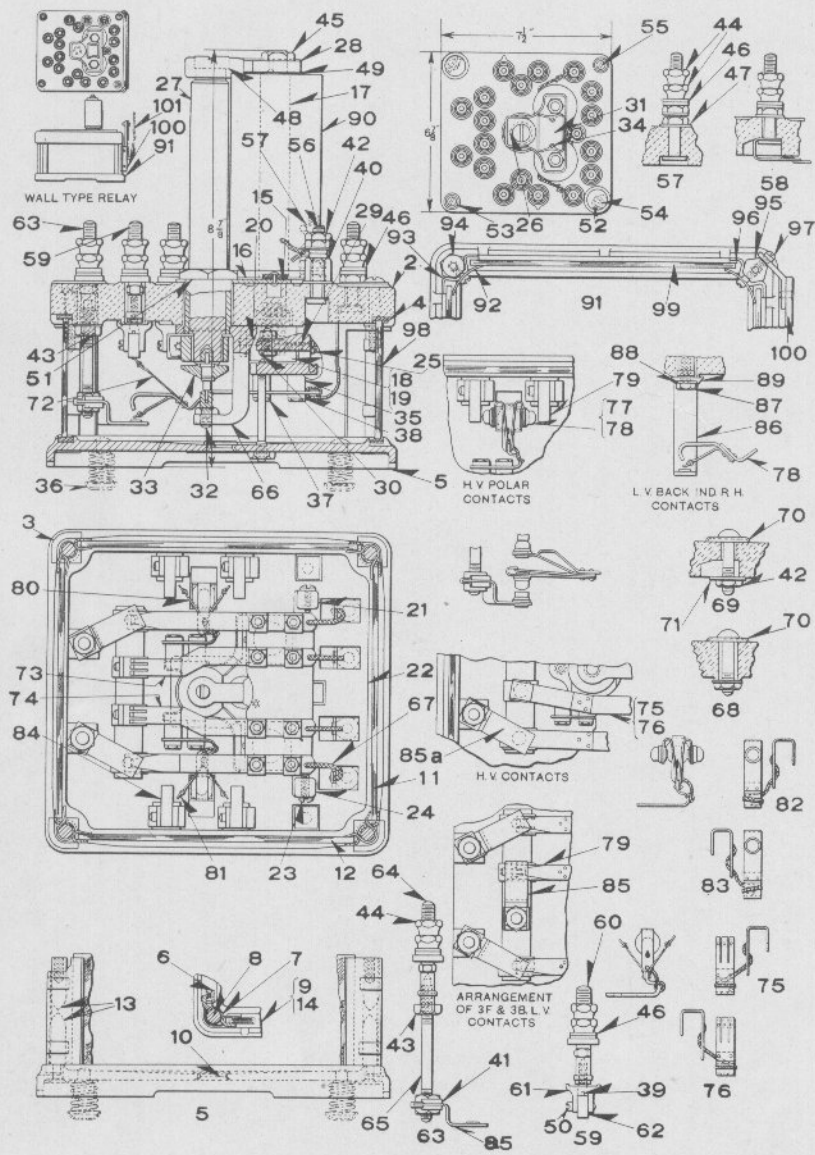
Details of the Model 12 Polarized Relay (Two Normal and Two Reverse Polar Contacts)
