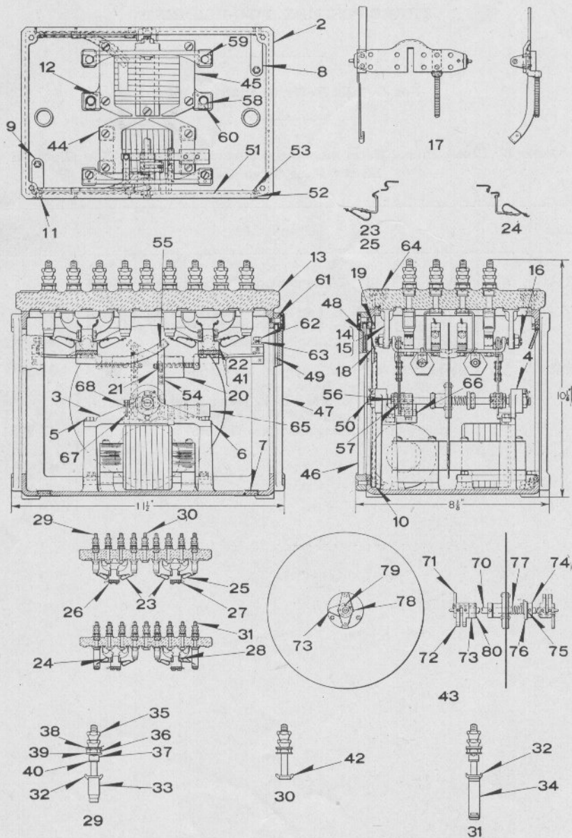
STYLE "TV-40" TWO-ELEMENT, THREE-POSITION VANE TYPE RELAY
