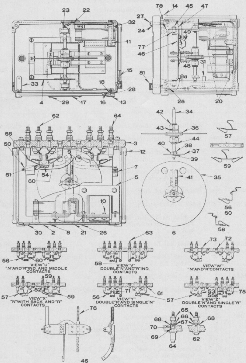
STYLE TV-30 THREE-POSITION VANE RELAY DETAILS
