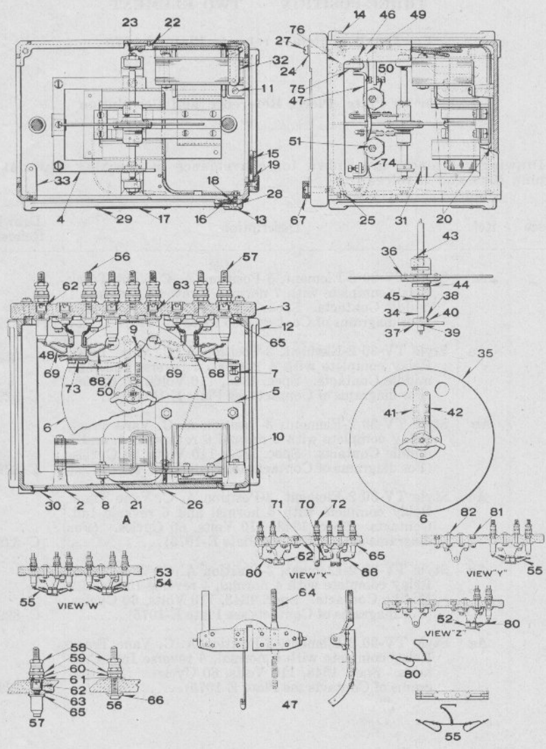
DETAILS OF STYLE TV-30 TWO-POSITION VANE RELAY
