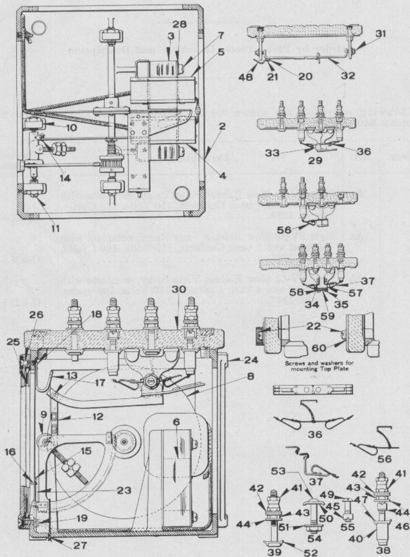
STYLE SV-32 SLOW RELEASE VANE RELAY DETAIL PARTS
