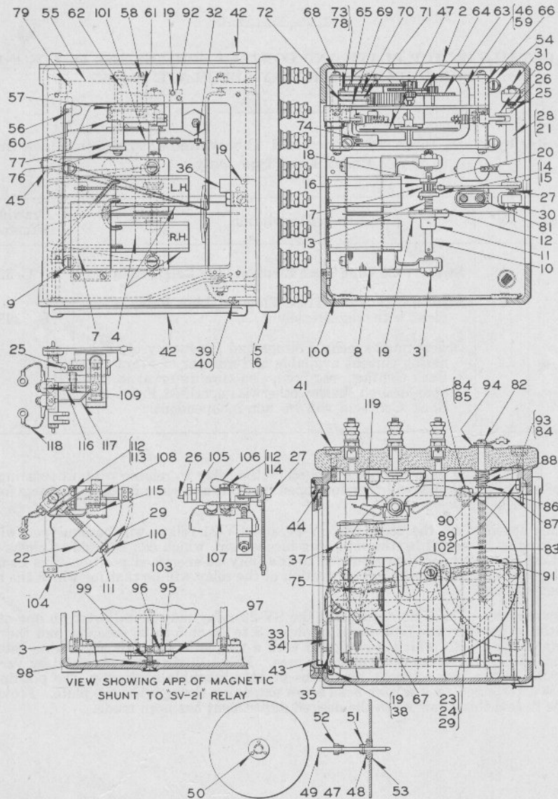
STYLE SV-20 AND SV-21 VANE TIME ELEMENT RELAYS (DETAIL PARTS)
