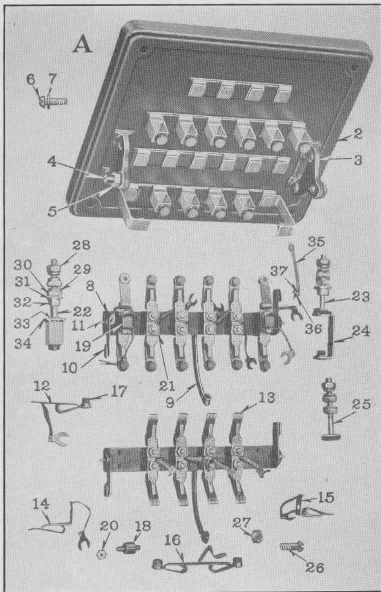
CIRCUIT CONTROLLING MECHANISM AND DETAILS FOR SV-12 AND TWO AND THREE POSITION MODEL 15 VANE RELAY
