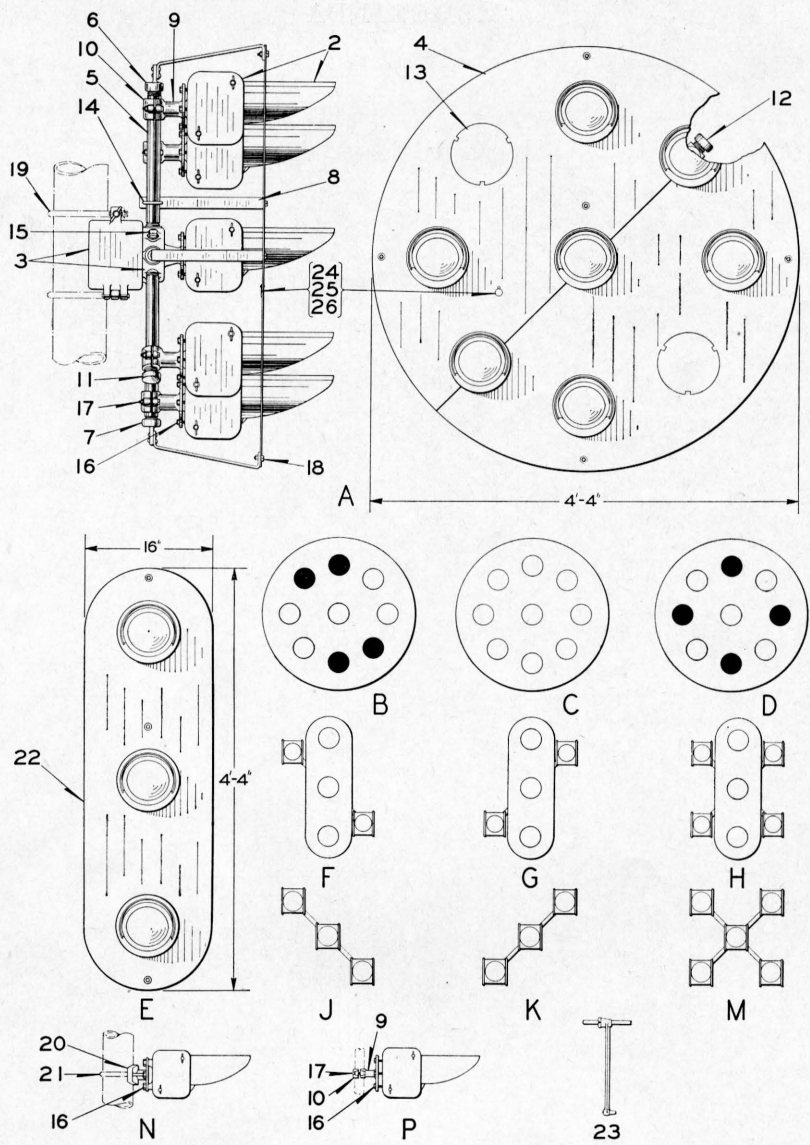
Style "PL-2" Position Light Signal Units with Lamp Units, Backgrounds, Terminal Boxes and Fittings for all arms of Ground, Bridge and Cantilever Mounted Signals.
