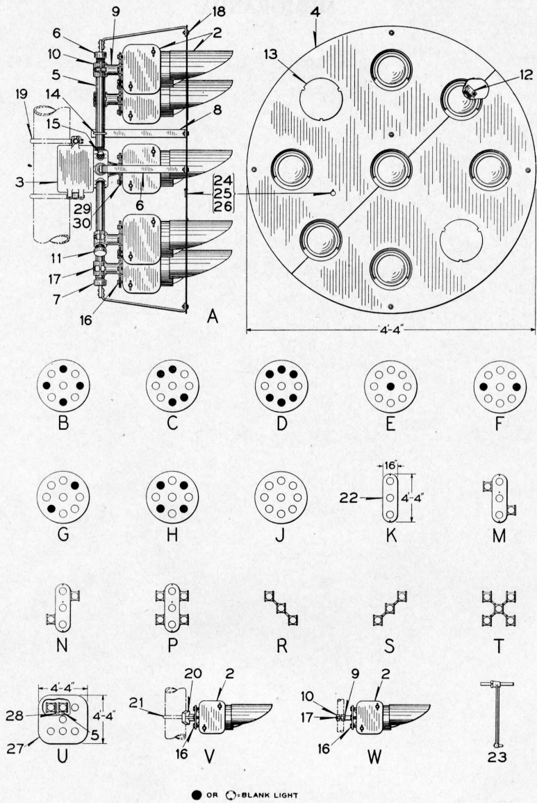
Style "PL-3" Position Light Signal Units with Lamp Units, Backgrounds, Terminal Boxes and Fittings for all Arms of Ground, Bridge and Cantilever Mounted Signals
