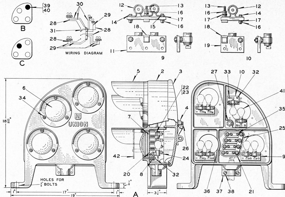
Position Light Dwarf Signal
