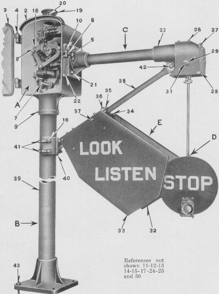
MAIN ASSEMBLIES AND DETAILS STYLE "DW" AUTOMATIC FLAGMAN (D-C.)
