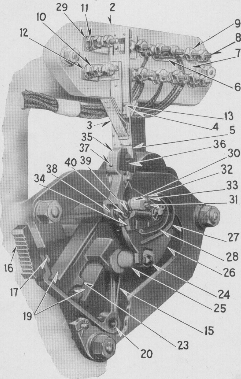
CIRCUIT CONTROLLER AND OPERATING ARM DETAILS STYLE "DW" AUTOMATIC FLAGMAN MECHANISM (D-C.)
