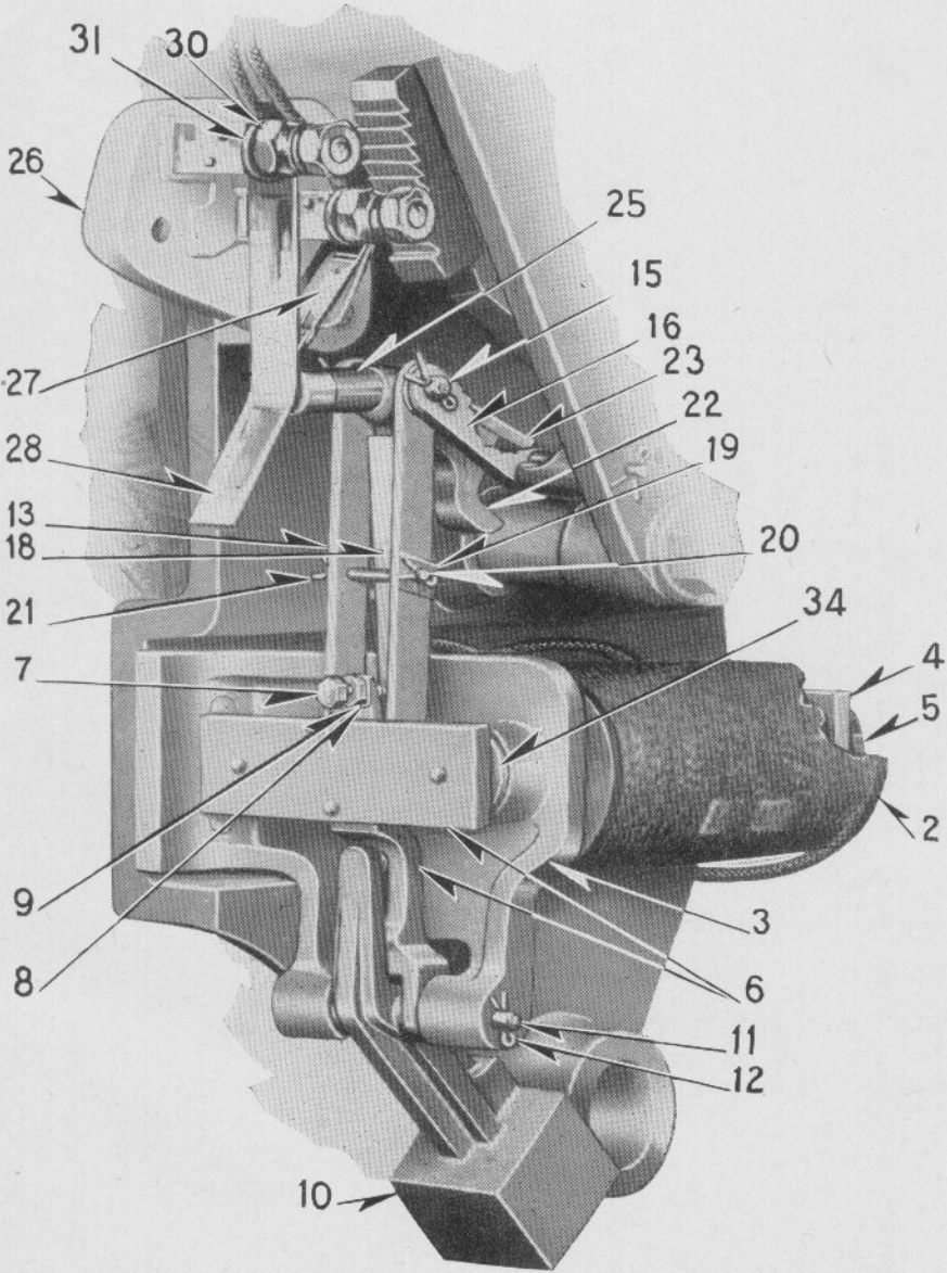
SLOT MAGNET DETAILS STYLE "DW" AUTOMATIC FLAGMAN MECHANISM (D-C.)
