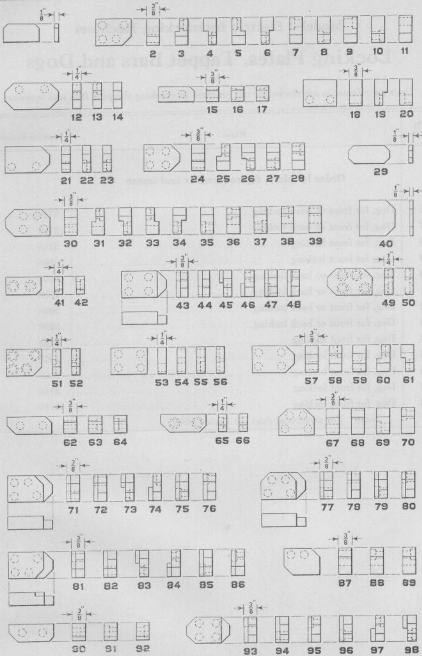
Locking Dogs For Model 2 Electric Interlocking Machines
