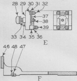
Lamp Cases For Model 5 Form A Electric Interlocking Machines
