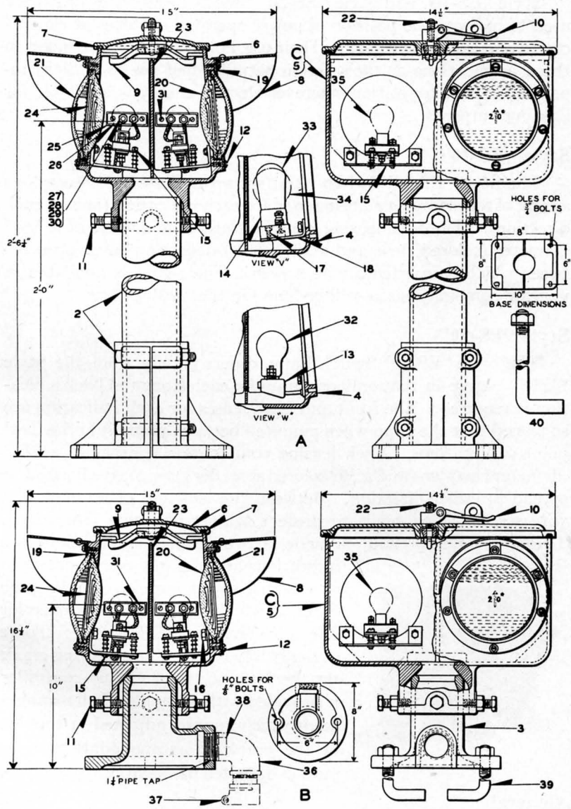
STYLE "ES-10" ELECTRIC SWITCH LAMP
