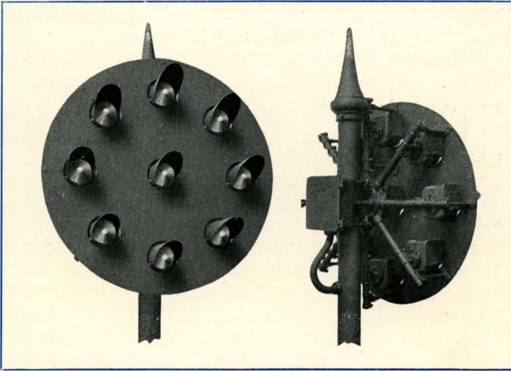
Figure 20 Type B Position-Light Signal Unit
