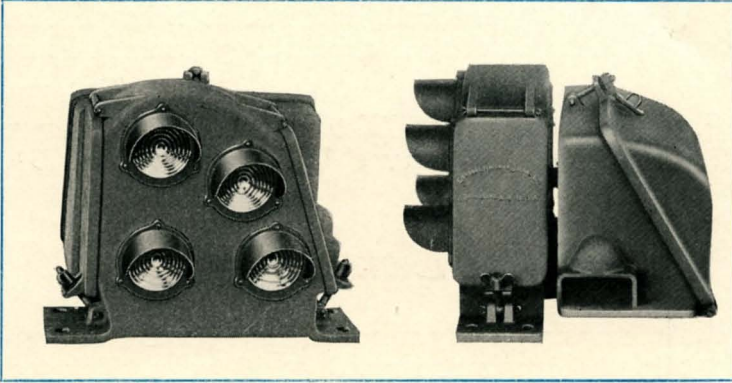
Figure 22 Type C Position-Light Dwarf Signal Unit
